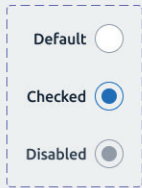
Radio button
