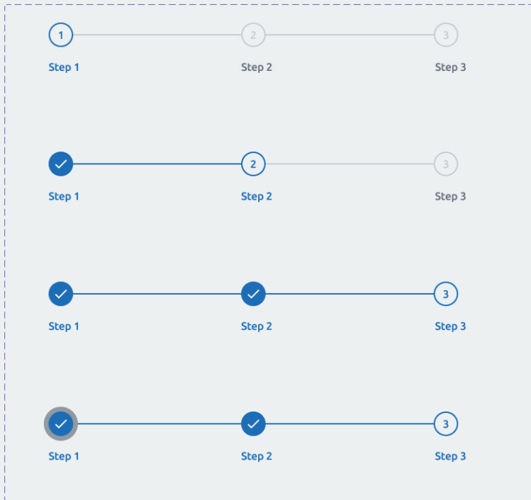
Progress bar
