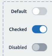
Toggle button
