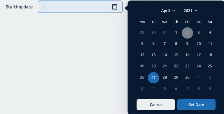
Date picker
